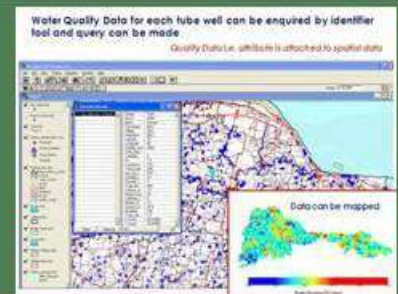
Bihar Ground Water Quality Mapping
